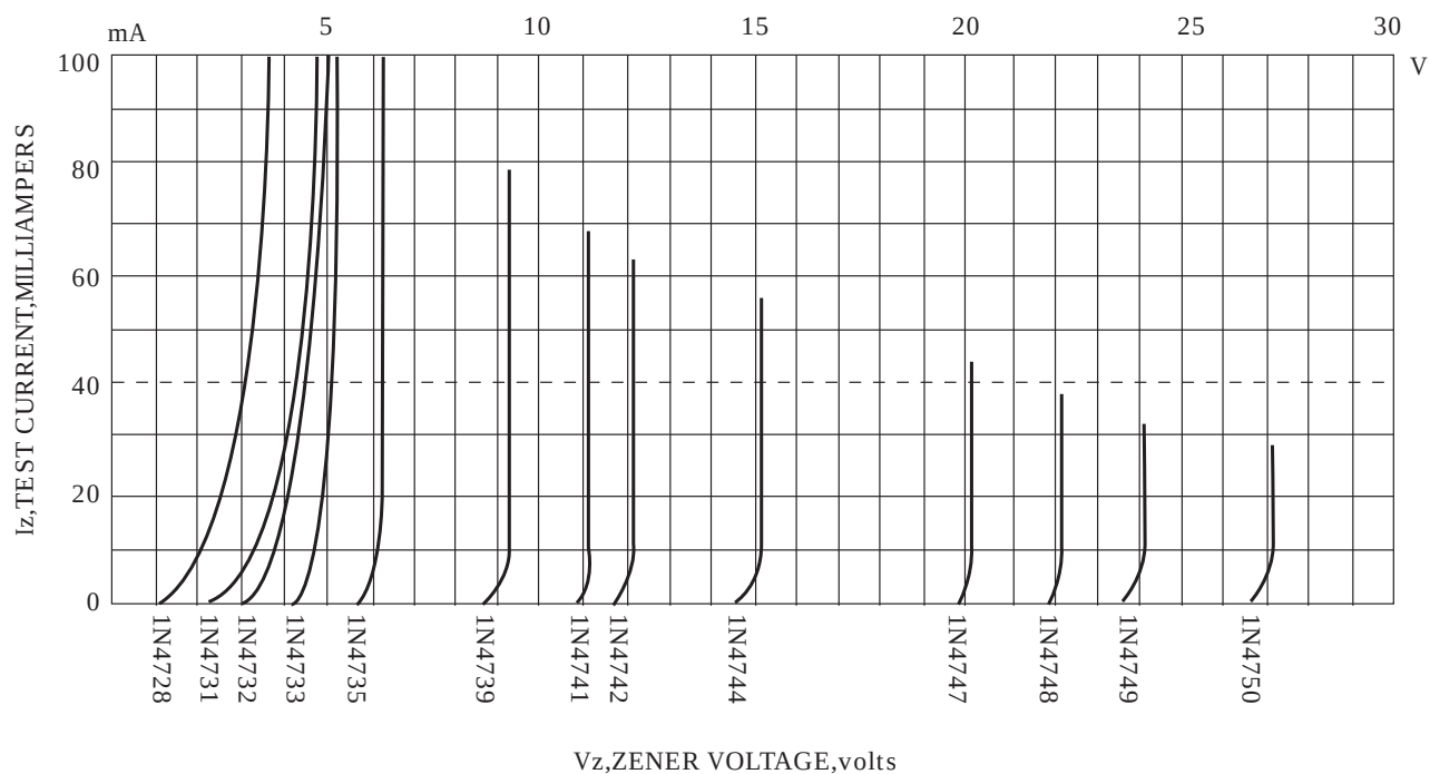
Breakdown characteristics
